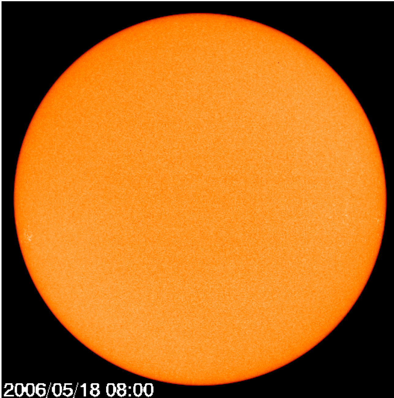
Visible (Red) Light View of the “Quiet” Sun – May 18, 2006
