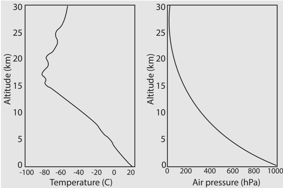
COSMIC satellite
